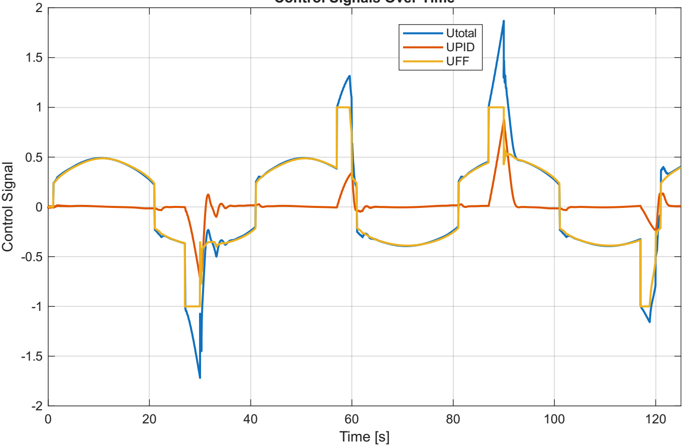
Control Signals Over Time
